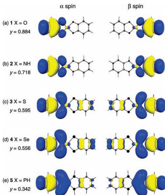
Figure 3. Magnetic orbitals for 1–5 calculated by the UHF/SDD+6–31G* method. The yellow and blue regions represent contour values of \pm 0.02 au, respectively.
