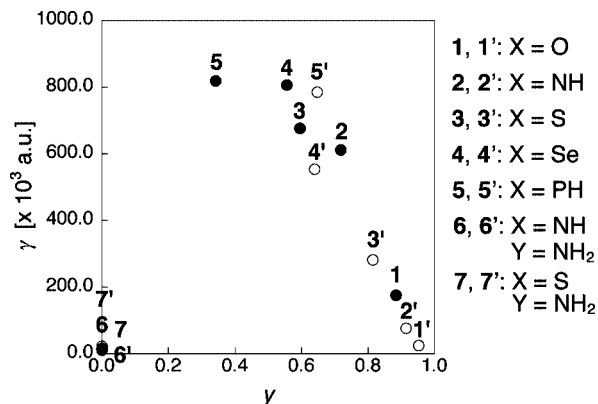
Figure 4. Diradical character ( \gamma ) dependence of \gamma [au] for original complexes 1–7 (●) and metal core eliminated complexes 1'–7' (○).
