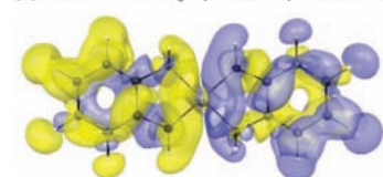
(b) 7 X, Y = S, NH 2 \gamma = 0.0 \gamma = 14 \times 10^3 a.u.
