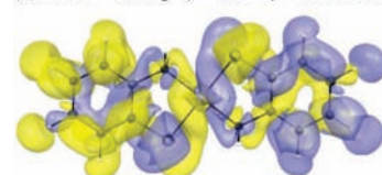
Figure 6. \gamma density distributions of 6 and 7 calculated by the RBHandHLYP/SDD+6–31G* method. The yellow and blue meshes represent positive and negative \gamma densities with contour values of \pm 10 au, respectively.
